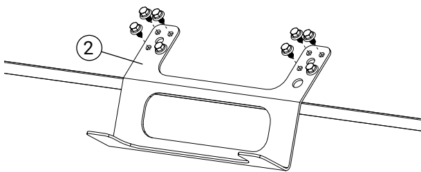
Installation of anti-slip protection directly on roof Direct installation on roof Fasteners: At least 8 x ≥ Ø5x25mm screws.
