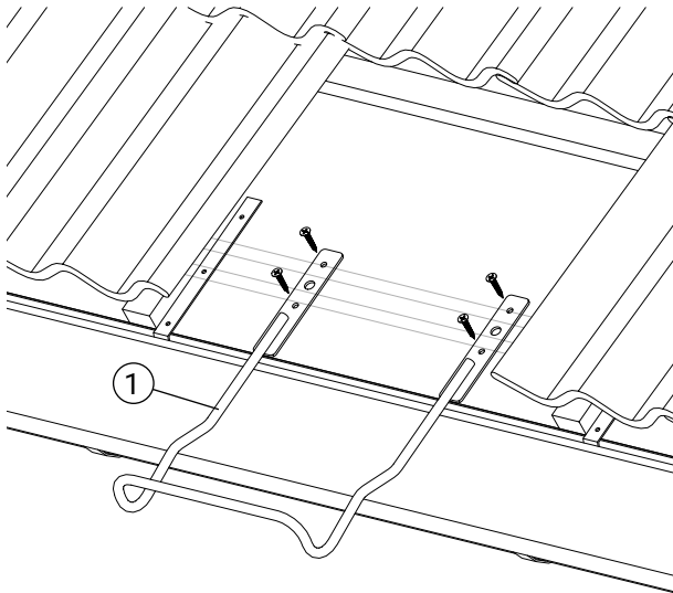
Installation of anti-slip protection using wood screw Fasteners: 4 x Ø5x25mm wood screws for grooved board.
