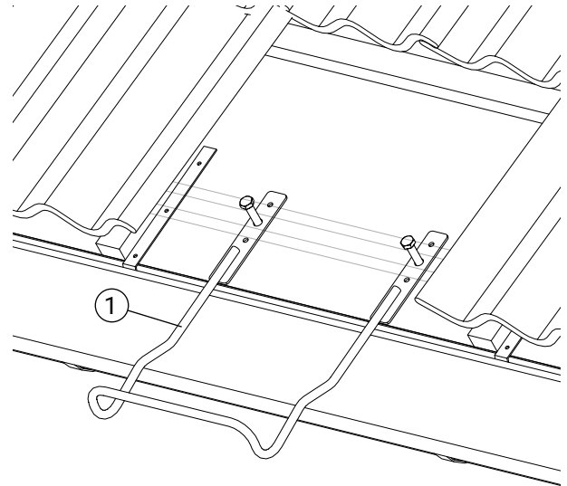
Installation of anti-slip protection with through bolt Through bolt on grooved board. Fasteners: 2 x M10 + nuts with washer.
