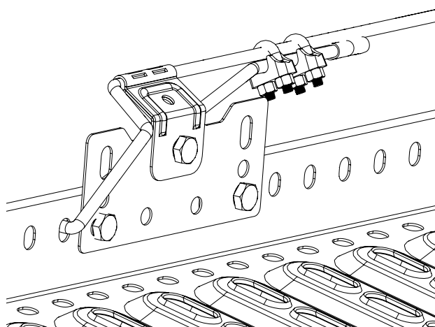
□ Weline ONE on roof bridge
