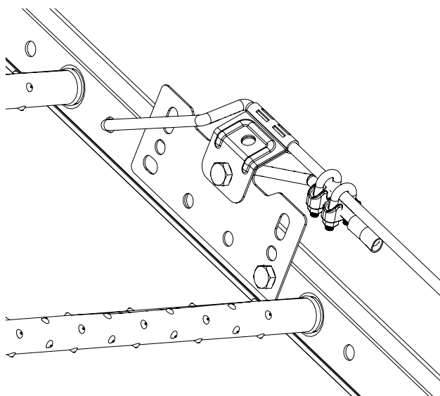
□ Weline ONE on roof ladder
